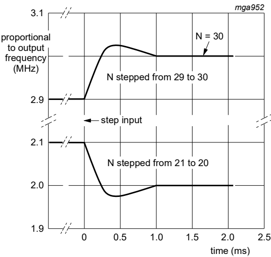
Fig. 38. Frequency compared to the time response
