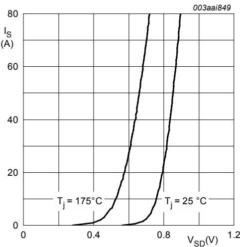
Fig. 16. Source-drain (diode forward) current as a function of source-drain (diode forward) voltage; typical values V_{GS} = 0V
