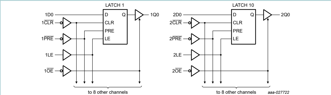
Fig. 3. Logic diagram
