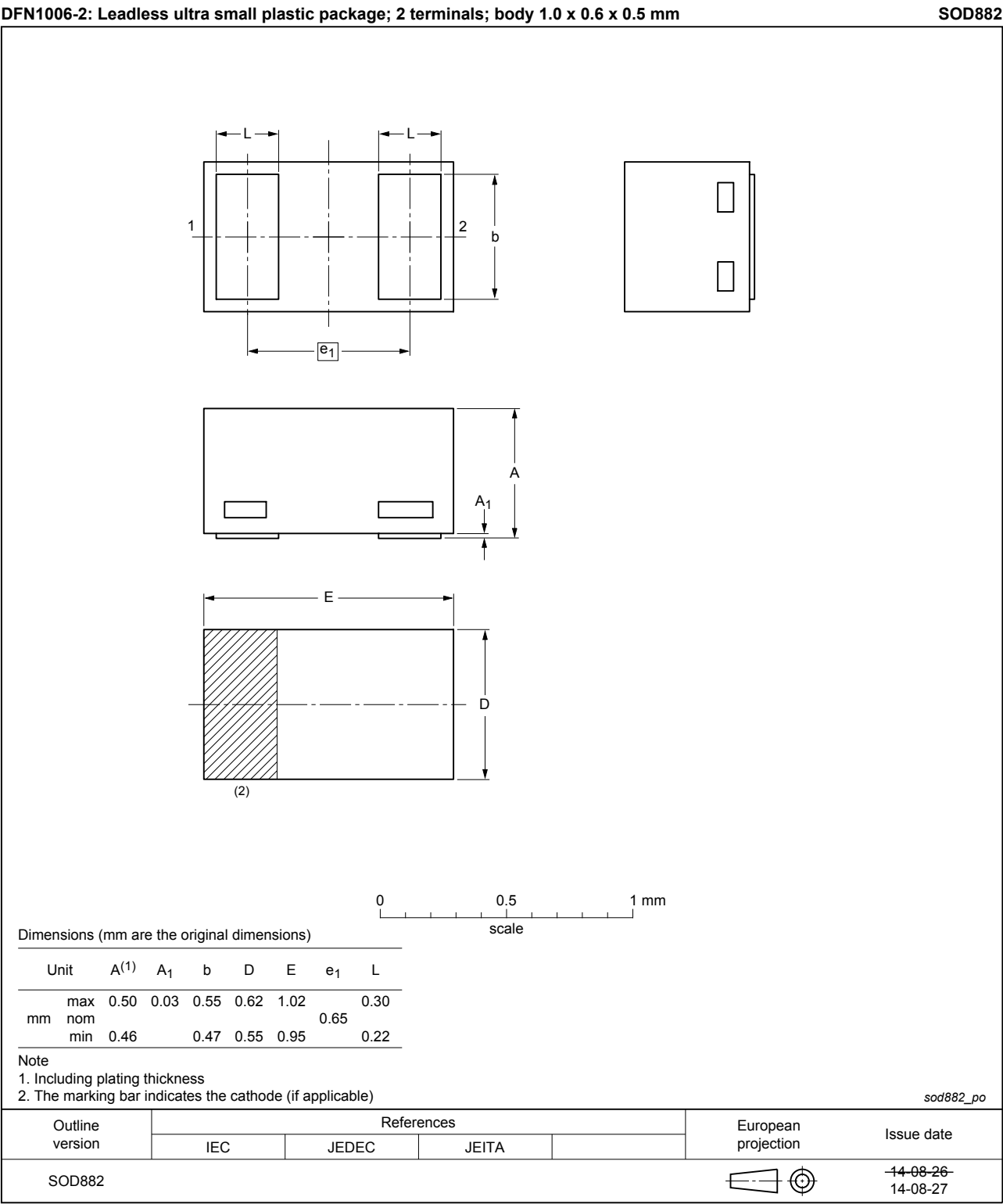
Fig. 10. Package outline DFN1006-2 (SOD882)
