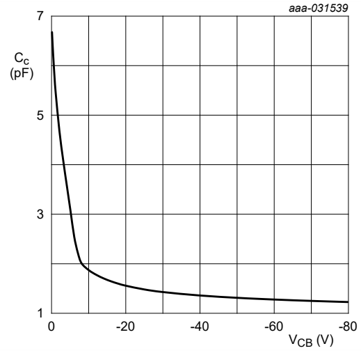
Fig. 9. NHDTA114EU: Collector capacitance as a function of collector-base voltage; typical values
