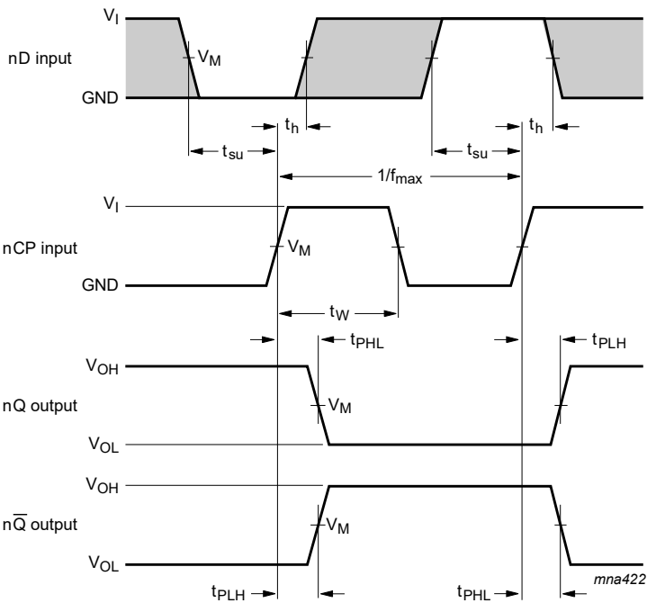
Measurement points are given in Table 8 . The shaded areas indicate when the input is permitted to change for predictable output performance. V OL and V OH are typical voltage output levels that occur with the output load.
