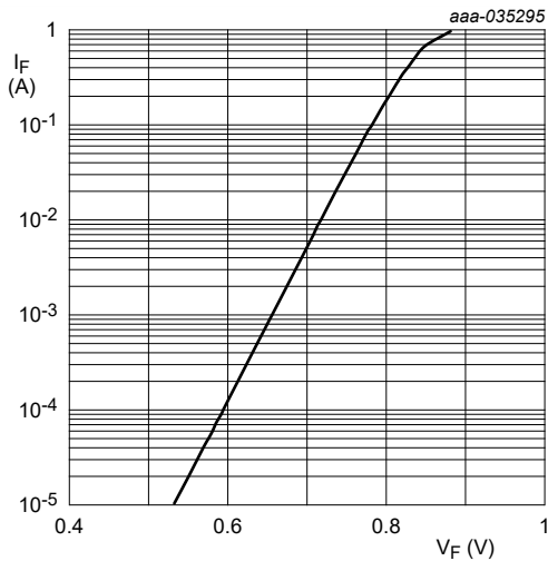
Fig. 5. Forward current as a function of forward voltage; typical values (HPZR-C5V6-Q)
