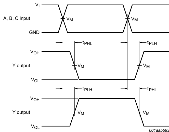
Fig. 9. Input A, B and C to output Y propagation delay times
