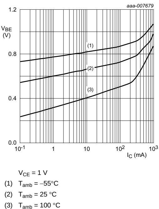
Fig 14. BC817-40QA: Base-emitter voltage as a function of collector current; typical values
