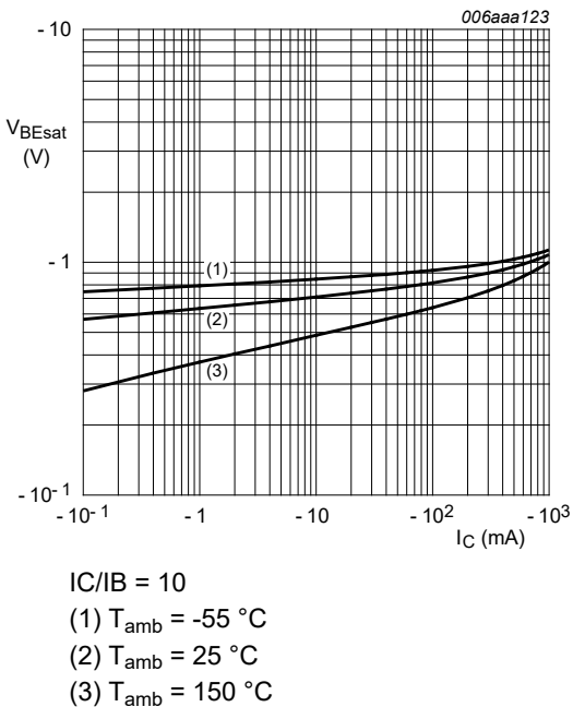
Fig. 10. BC807-25QB: Base-emitter saturation voltage as a function of collector current; typical values
