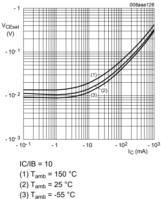
Fig. 11. BC807-25QB: Collector-emitter saturation voltage as a function of collector current; typical values
