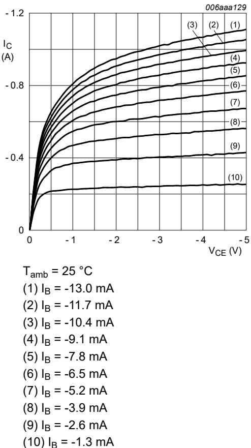
Fig. 9. BC807-25QB: Collector current as a function of collector-emitter voltage; typical values
