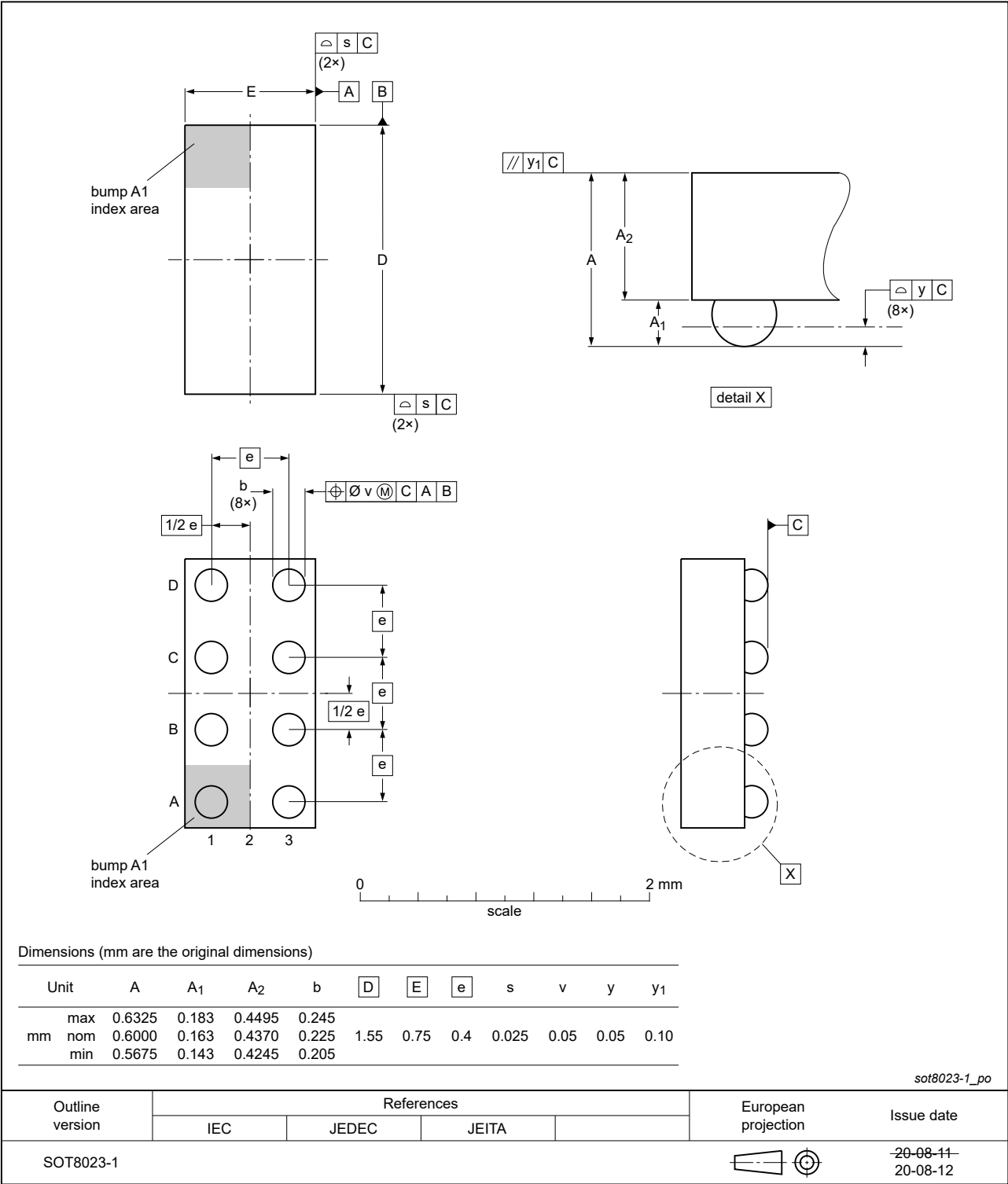
Fig. 11. Package outline SOT8023-1 (WLCSP8)
