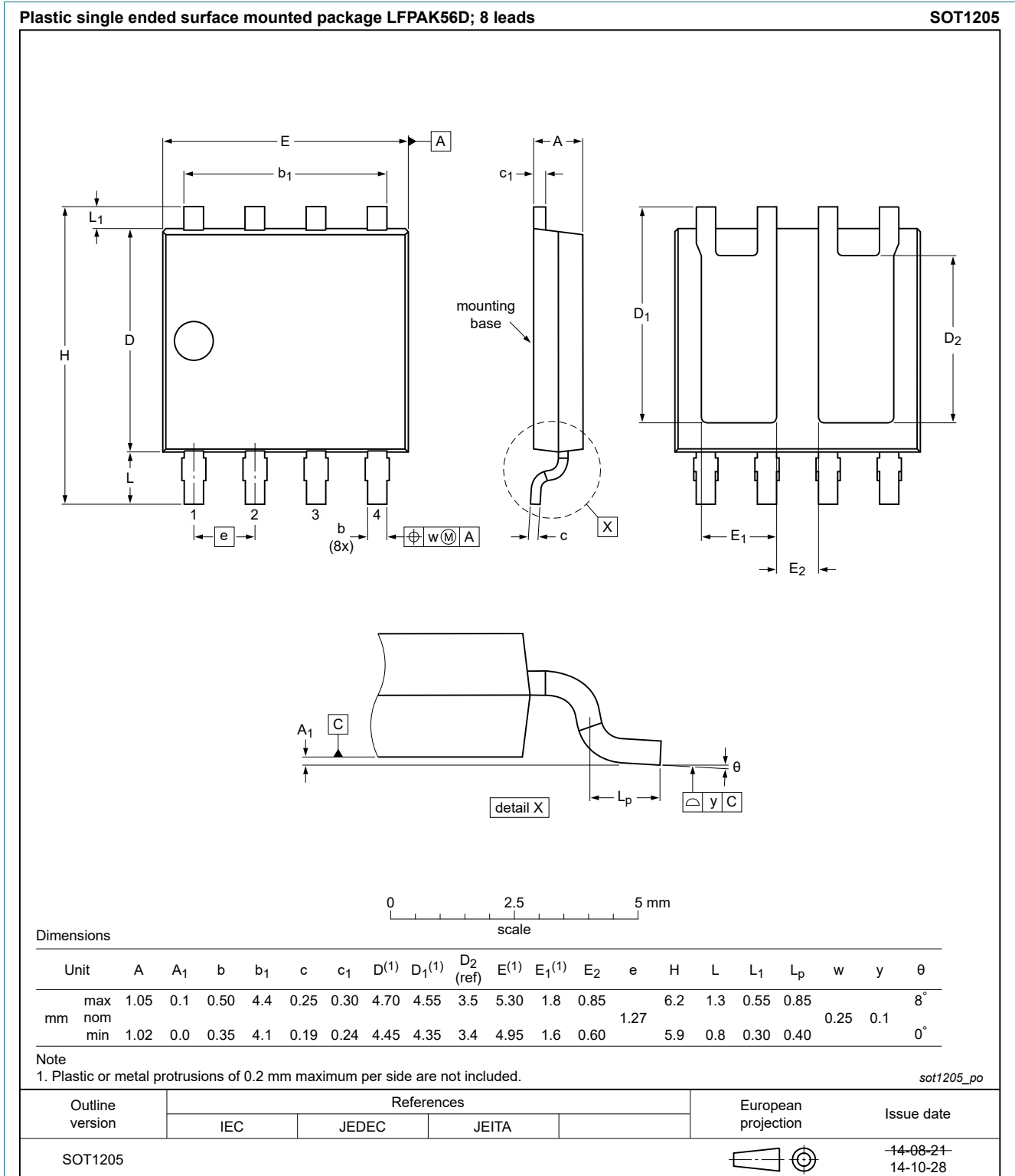
Fig. 17. Package outline LPAK56D; Dual LPAK (SOT1205)
