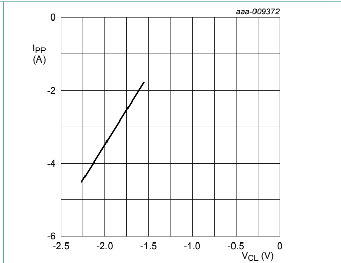
IEC 61000-4-5; t_p = 8/20 \mu s ; negative pulse
