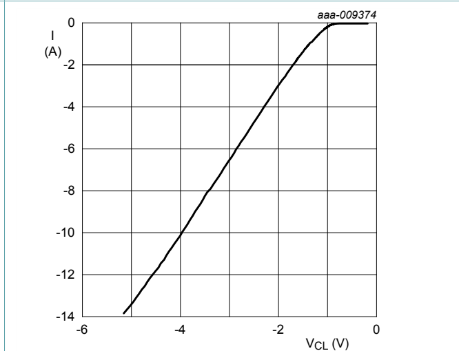
t_p = 100 ns ; Transmission Line Pulse (TLP)
