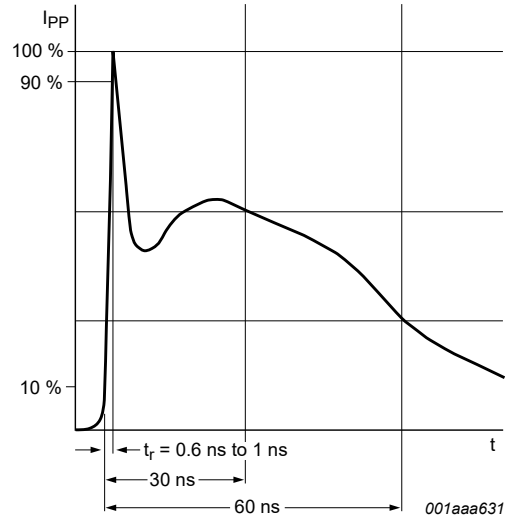
Fig. 3. ESD pulse waveform according to IEC 61000-4-2
