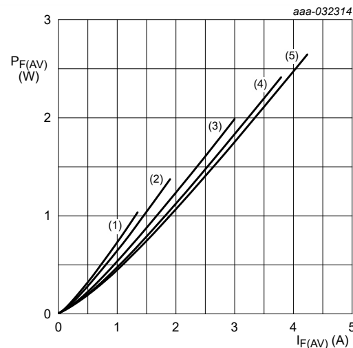
T_j = 100\text{ }^{\circ}\text{C} (1) \delta = 0.1 (2) \delta = 0.2 (3) \delta = 0.5 (4) \delta = 1 ; DC (5) \delta = 1 ; DC
