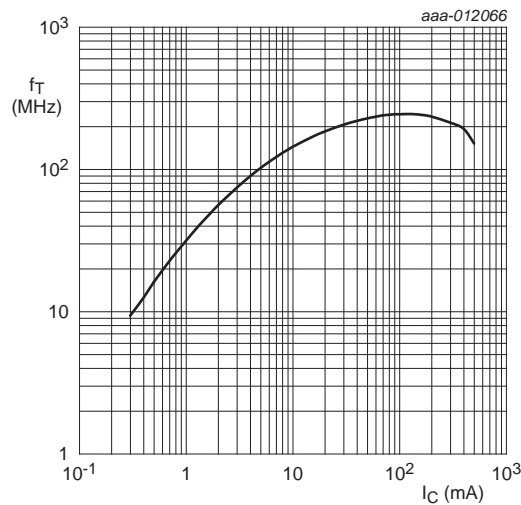
Fig 24. PDTD114ET: Transition frequency as a function of collector current; typical values of built-in transistor
