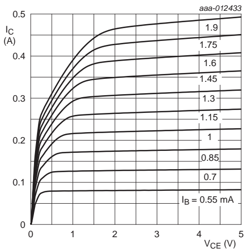
Fig 22. PDTD123EU: Collector current as a function of collector-emitter voltage; typical values
