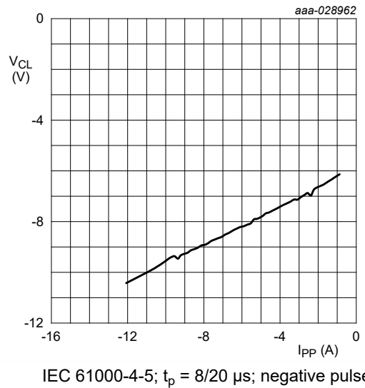
Fig. 8. Negative clamping voltage (8/20 \mu s pulse); typical values
