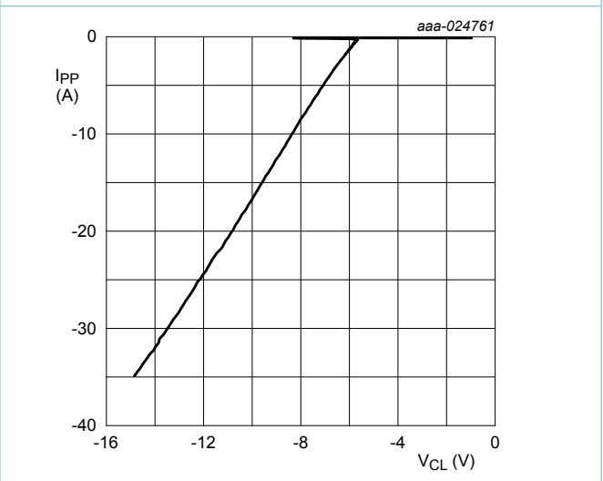
Fig. 6. Negative clamping voltage (TLP); typical values t p = 100 ns; Transmission Line Pulse (TLP)
