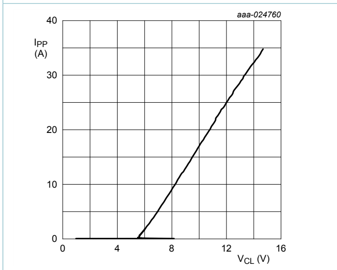
Fig. 5. Positive clamping voltage (TLP); typical values t p = 100 ns; Transmission Line Pulse (TLP)
