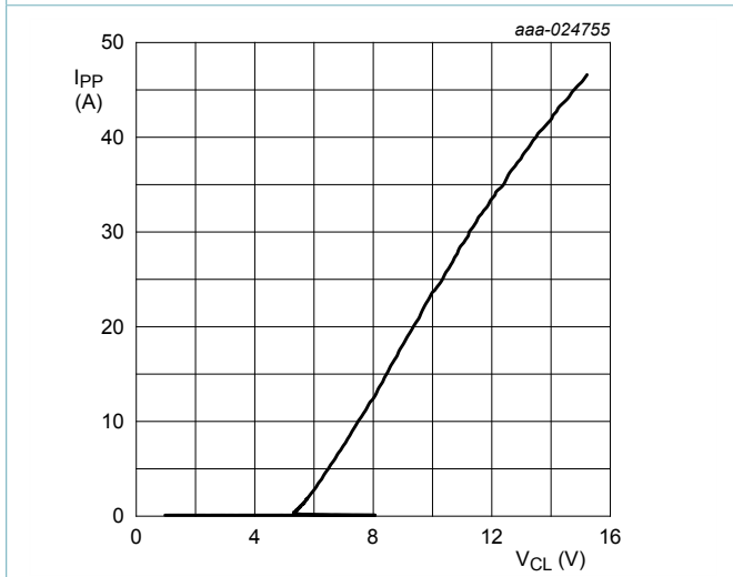
Fig. 5. Positive clamping voltage (TLP); typical values t p = 100 ns; Transmission Line Pulse (TLP)
