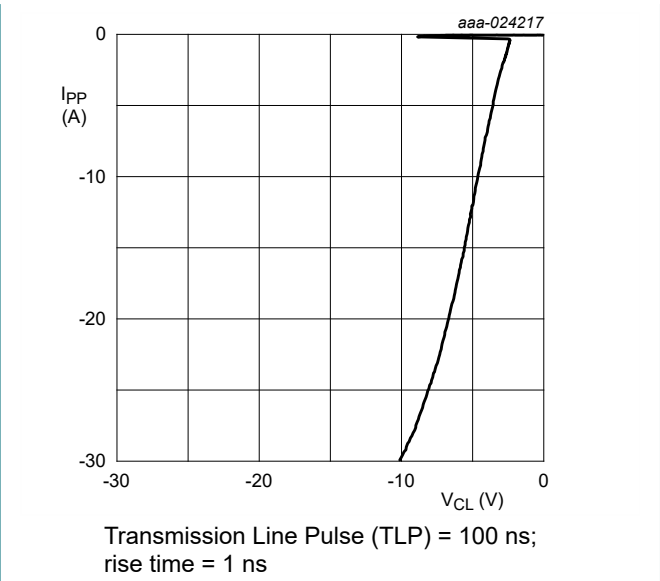
Fig. 13. Negative clamping voltage (TLP); typical values
