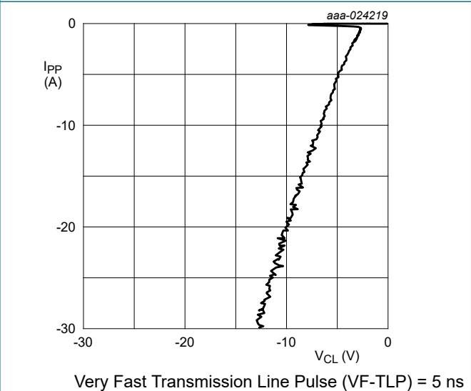
Fig. 15. Negative clamping voltage (VF-TLP); typical values
