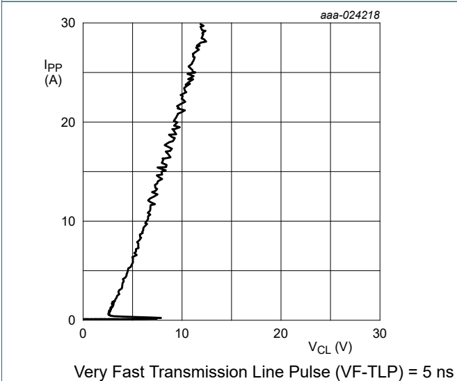
Fig. 14. Positive clamping voltage (VF-TLP); typical values
