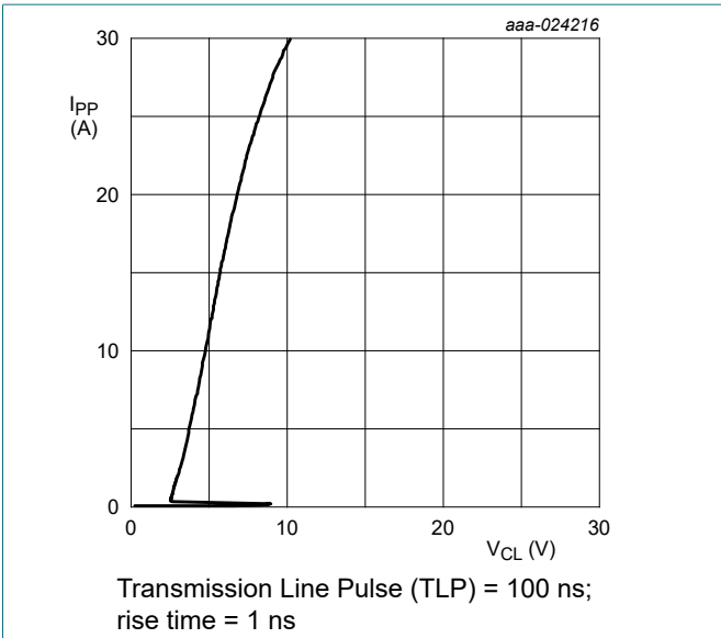
Fig. 12. Positive clamping voltage (TLP); typical values
