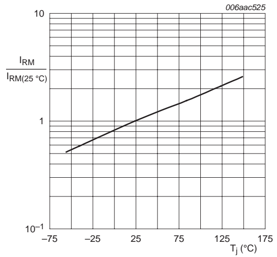
Fig 5. Relative variation of reverse leakage current as a function of junction temperature; typical values
