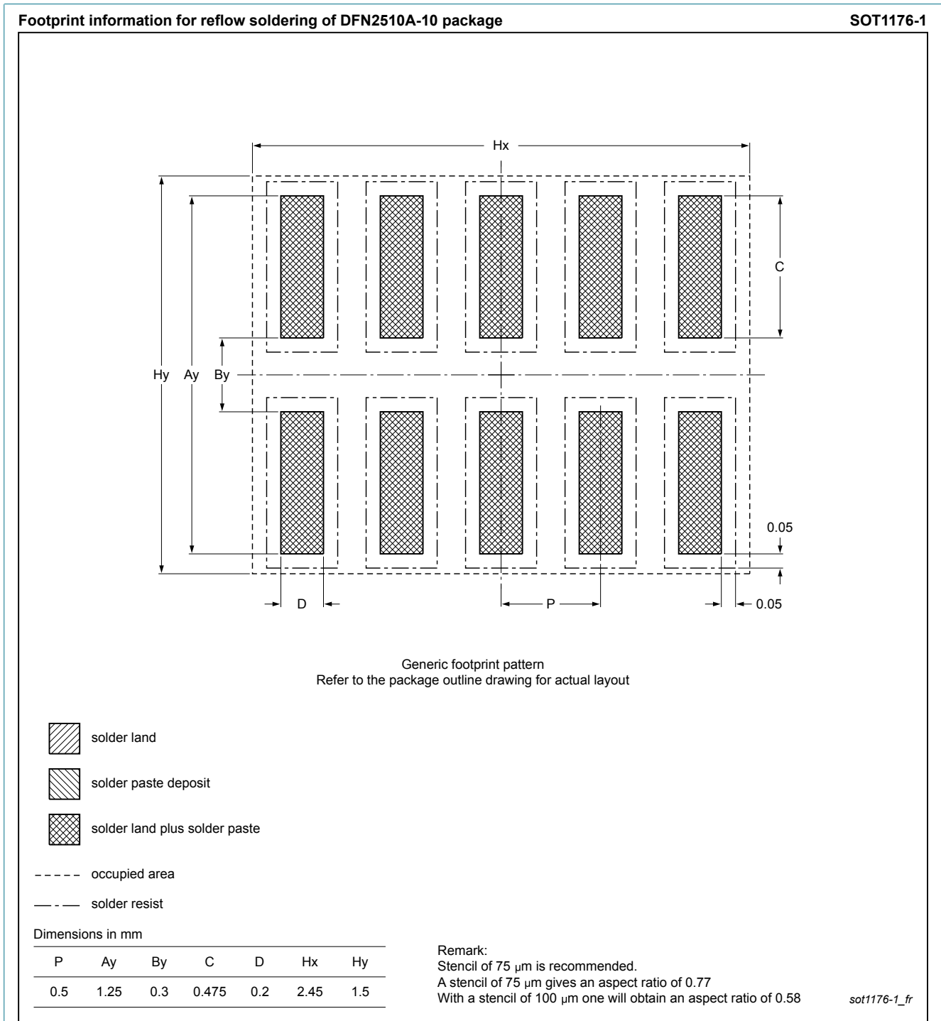
Fig. 14. Reflow soldering footprint for DFN2510A-10 (SOT1176-1)
