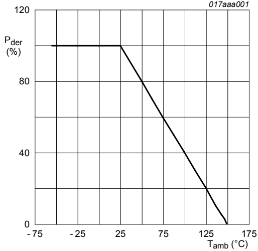
Fig. 2. Normalized total power dissipation as a function of ambient temperature
