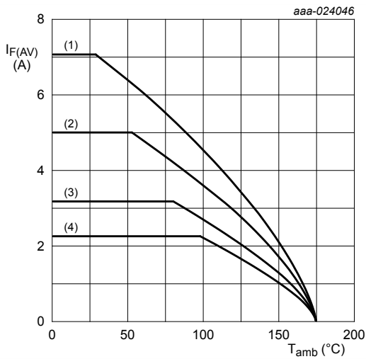
FR4 PCB, mounting pad for cathode 1\text{ cm}^2 T_j = 175^\circ\text{C} (1) \delta = 1 ; DC (2) \delta = 0.5 ; f = 20\text{ kHz} (3) \delta = 0.2 ; f = 20\text{ kHz} (4) \delta = 0.1 ; f = 20\text{ kHz}
