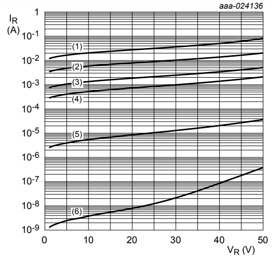
pulsed condition (1) T_j = 150^\circ\text{C} (2) T_j = 125^\circ\text{C} (3) T_j = 100^\circ\text{C} (4) T_j = 85^\circ\text{C} (5) T_j = 25^\circ\text{C} (6) T_j = -40^\circ\text{C}
