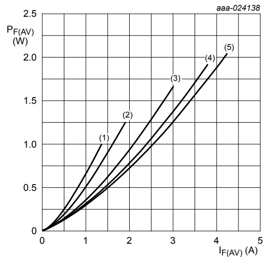
T_j = 100^\circ\text{C} (1) \delta = 0.1 (2) \delta = 0.2 (3) \delta = 0.5 (4) \delta = 0.8 (5) \delta = 1
