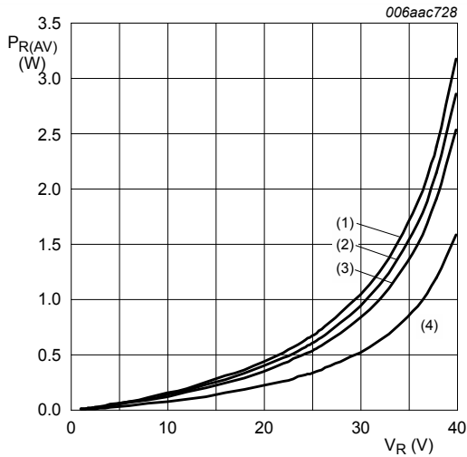
T_j = 150\text{ °C} (1) \delta = 1.0 (2) \delta = 0.9 (3) \delta = 0.8 (4) \delta = 0.5
