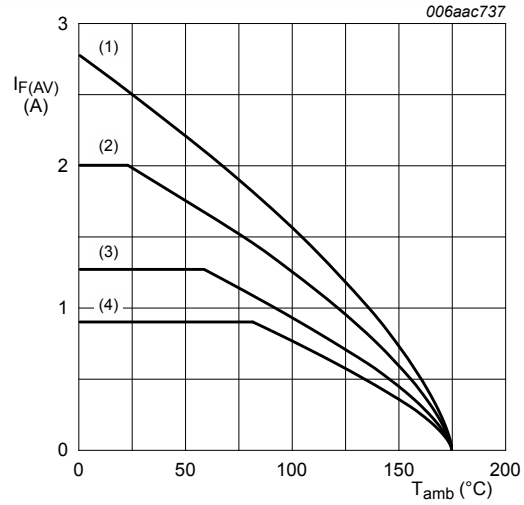
FR4 PCB, standard footprint T_j = 175\text{ }^\circ\text{C} (1) \delta = 1.0 (DC) (2) \delta = 0.5 ; f = 20\text{ kHz} (3) \delta = 0.2 ; f = 20\text{ kHz} (4) \delta = 0.1 ; f = 20\text{ kHz}
