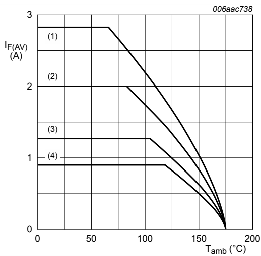
FR4 PCB, mounting pad for cathode 1\text{ cm}^2 T_j = 175\text{ }^\circ\text{C} (1) \delta = 1.0 (DC) (2) \delta = 0.5 ; f = 20\text{ kHz} (3) \delta = 0.2 ; f = 20\text{ kHz} (4) \delta = 0.1 ; f = 20\text{ kHz}
