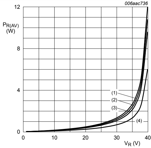
T_j = 150\text{ }^\circ\text{C} (1) \delta = 1.0 (2) \delta = 0.9 (3) \delta = 0.8 (4) \delta = 0.5
