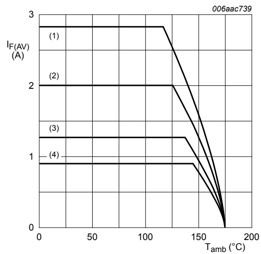
Ceramic PCB, \text{Al}_2\text{O}_3 , standard footprint T_j = 175\text{ }^\circ\text{C} (1) \delta = 1.0 (DC) (2) \delta = 0.5 ; f = 20\text{ kHz} (3) \delta = 0.2 ; f = 20\text{ kHz} (4) \delta = 0.1 ; f = 20\text{ kHz}
