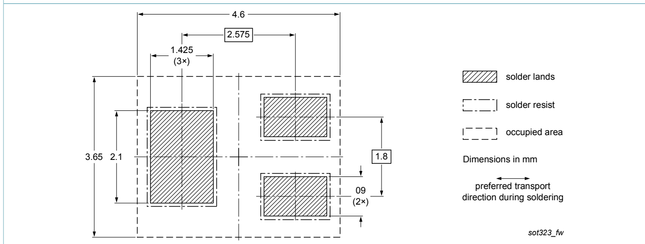
Fig. 20. Wave soldering footprint for SC-70 (SOT323)
