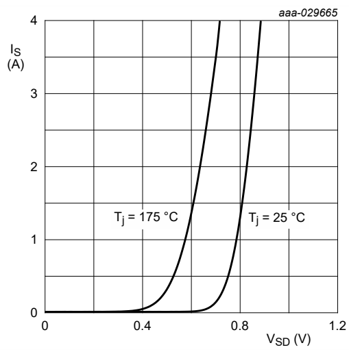
V_{GS} = 0 V Fig. 16. Source current as a function of source-drain voltage; typical values
