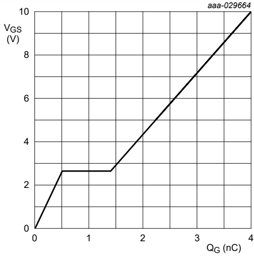
V_{DS} = 30 V; I_D = 2.2 A Fig. 14. Gate-source voltage as a function of gate charge; typical values
