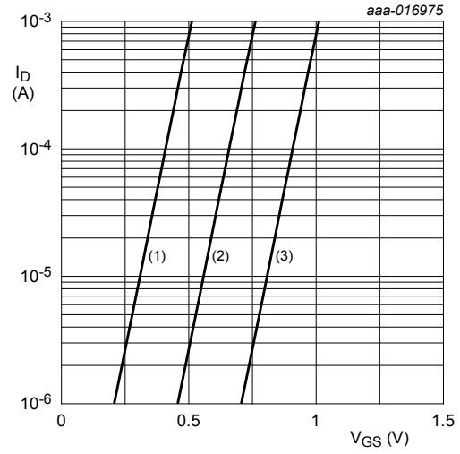
Fig. 7. Sub-threshold drain current as a function of gate-source voltage T_j = 25\text{ °C} ; V_{DS} = 5\text{ V} (1) minimum values (2) typical values (3) maximum values
