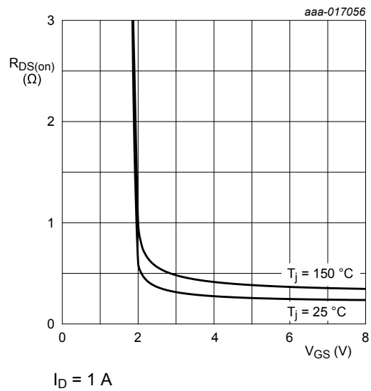
Fig. 10. Drain-source on-state resistance as a function of gate-source voltage; typical values I_D = 1 \text{ A}
