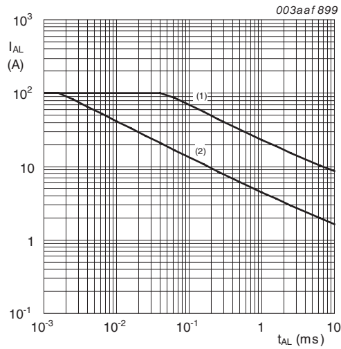
(1) T_{j (trnt)} = 25^\circ C ; (2) T_{j (trnt)} = 100^\circ C
