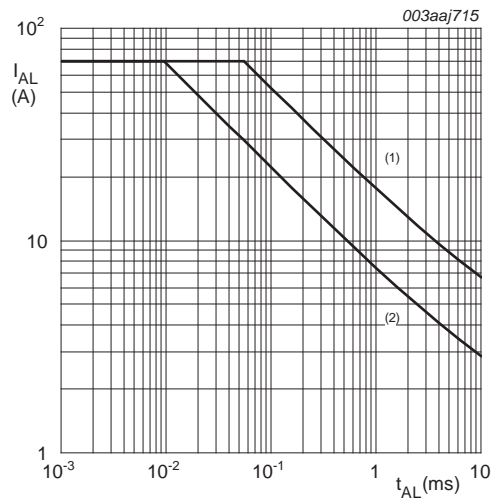
(1) T_{j(jmb)} = 25^{\circ}C ; (2) T_{j(jmb)} = 100^{\circ}C
