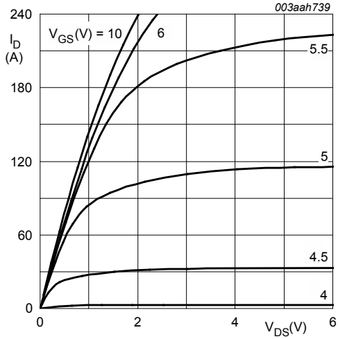
Fig. 6. Output characteristics; drain current as a function of drain-source voltage; typical values T_j = 25\text{ °C}; t_p = 300\ \mu\text{s}
