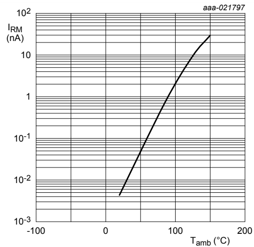
Fig. 7. Relative variation of reverse leakage current as a function of ambient temperature; typical values V_{RWM} = 15\text{ V}
