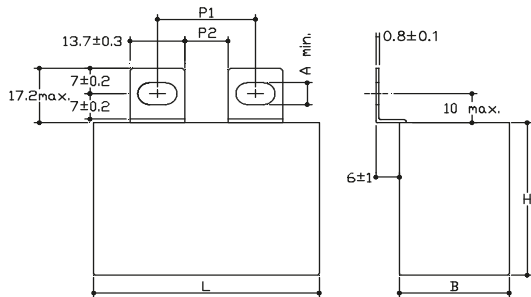
Fixing pitch and distance between lugs (mm)
