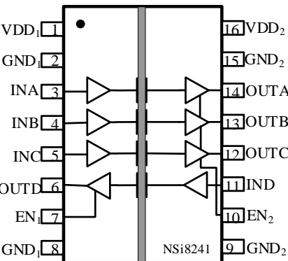
Figure 1.2 NSi8241W Package
