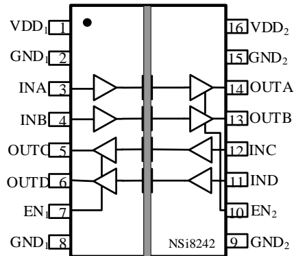
Figure 1.3 NSi8242W Package
