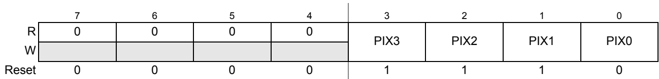
Figure 5-8. Program Page Index Register (PPAGE)
