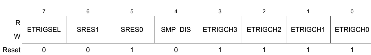
Figure 15-4. ATD Control Register 1 (ATDCTL1)
