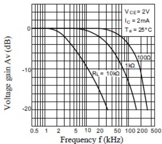
Fig.9 Frequency Response
