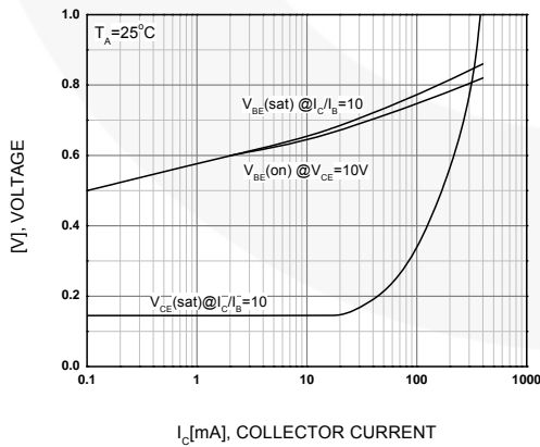
Figure 5. On Voltage
