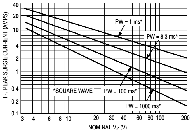
Figure 5. Maximum Non-Repetitive Surge Current versus Nominal Zener Voltage (See Note 4)
