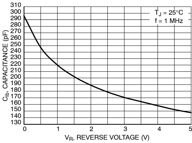
Figure 9. Input Capacitance
