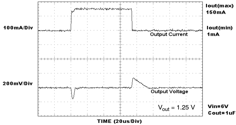
Figure 31. Load Transient Response (1.0 μF)
