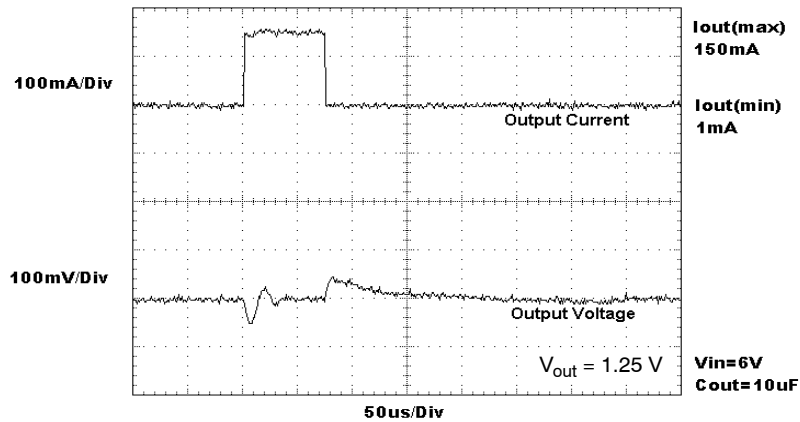
Figure 32. Load Transient Response (10 μF)
