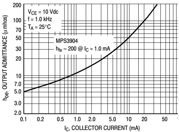
Figure 18. Output Admittance
