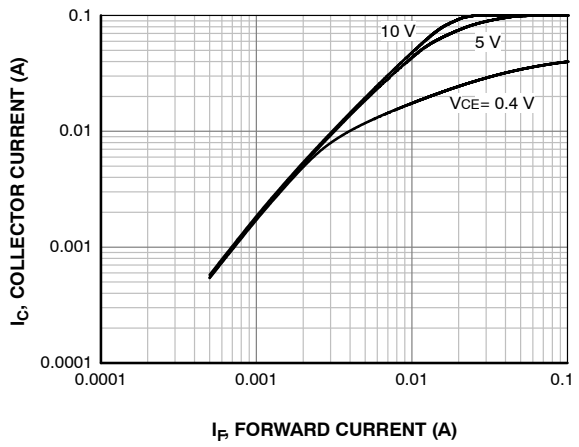
Figure 8. Collector Current vs. Forward Current
