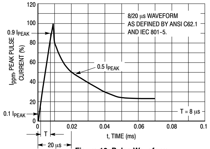
Figure 10. Pulse Waveform
