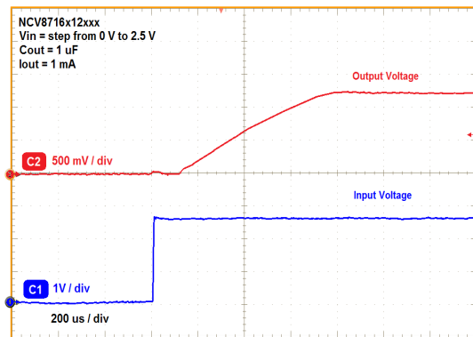
Figure 38. Input Voltage Turn-On Response
