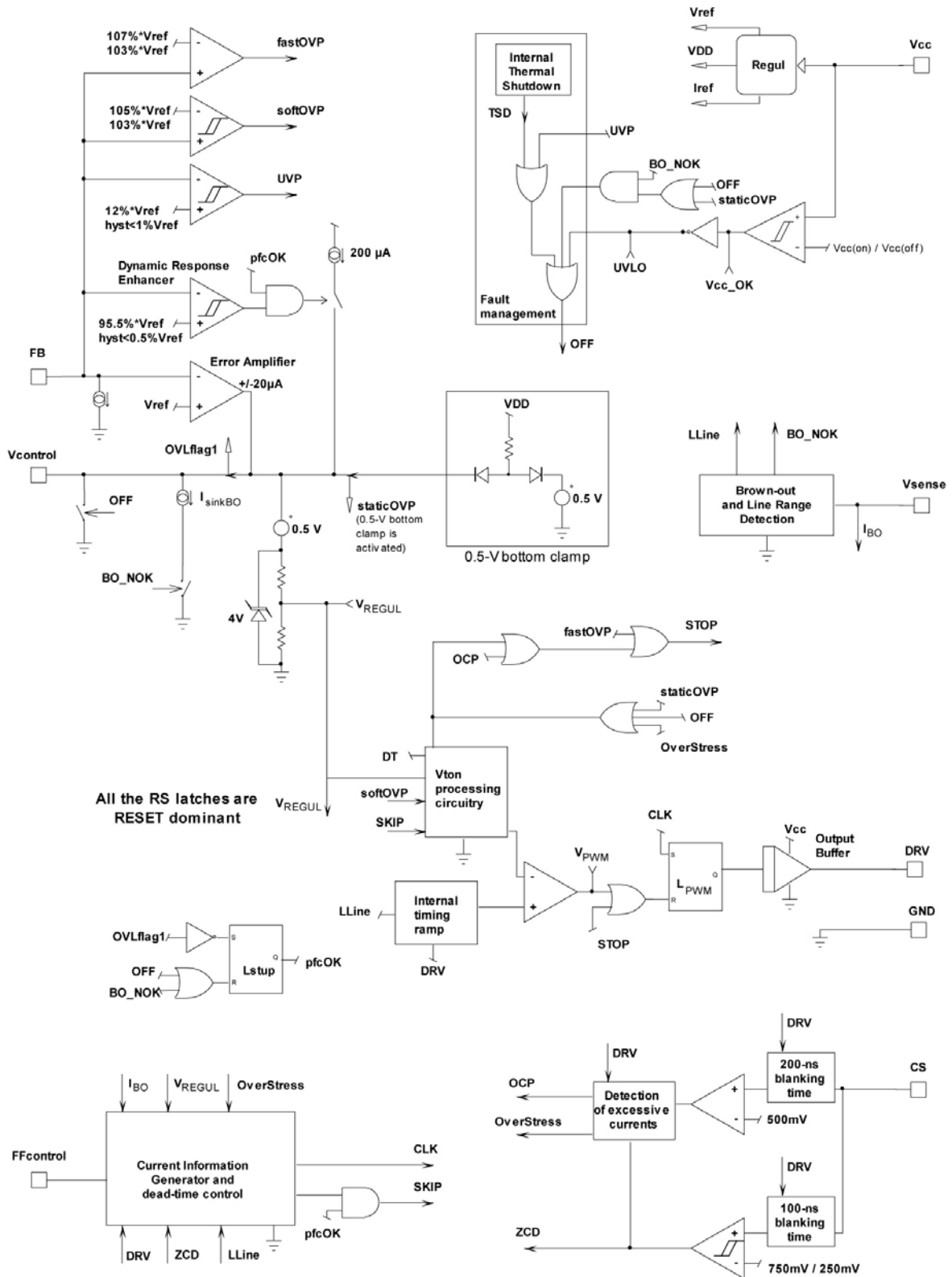
Figure 2. Block Diagram
