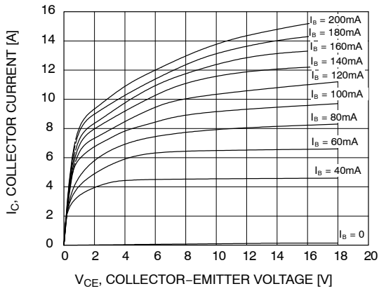
Figure 1. Static Characteristic
